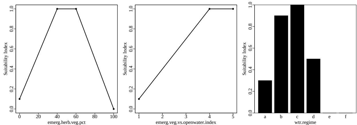
Figure 1. Suitability index graphs for variables included in the americancoot model in ecorest .
