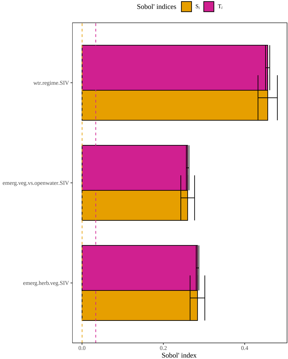
Figure 4. Results of a sensitivity analysis for the americancoot model based on an arithmetic mean structure. Dashed lines represent baseline numerical approximation error for S_i and T_i ( i.e. , dummy variables).
